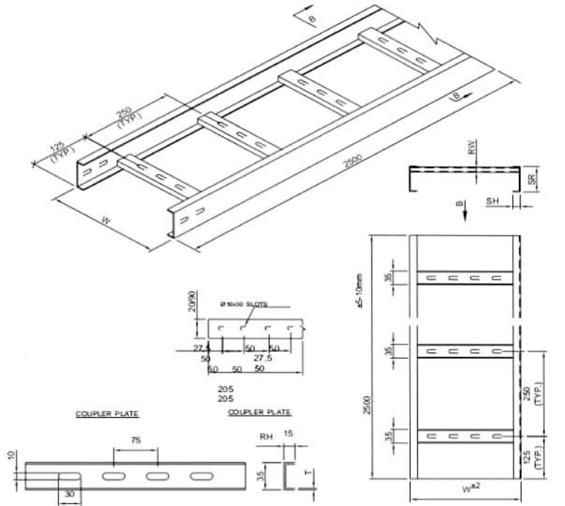
LADDER TYPE CABLE TRAY
